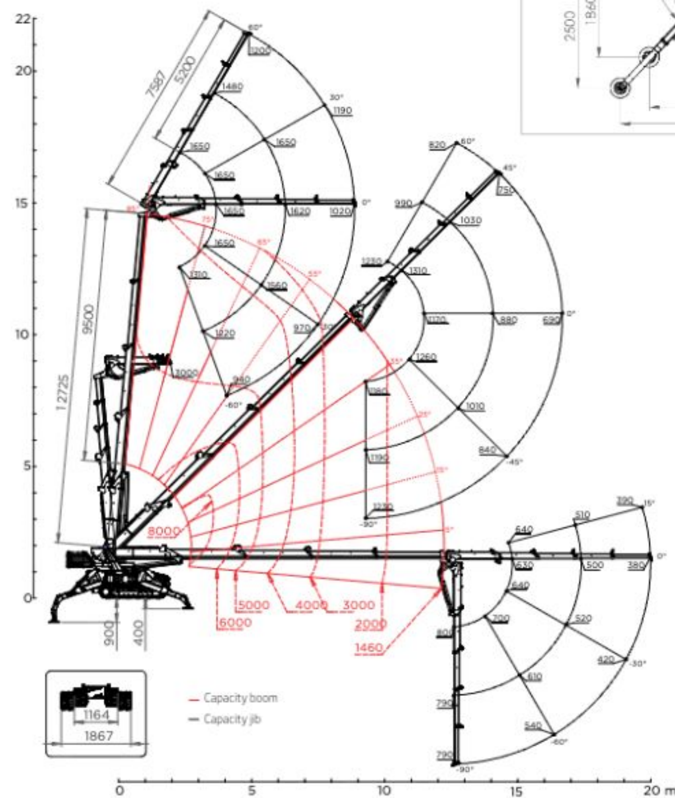
Standard with jib
