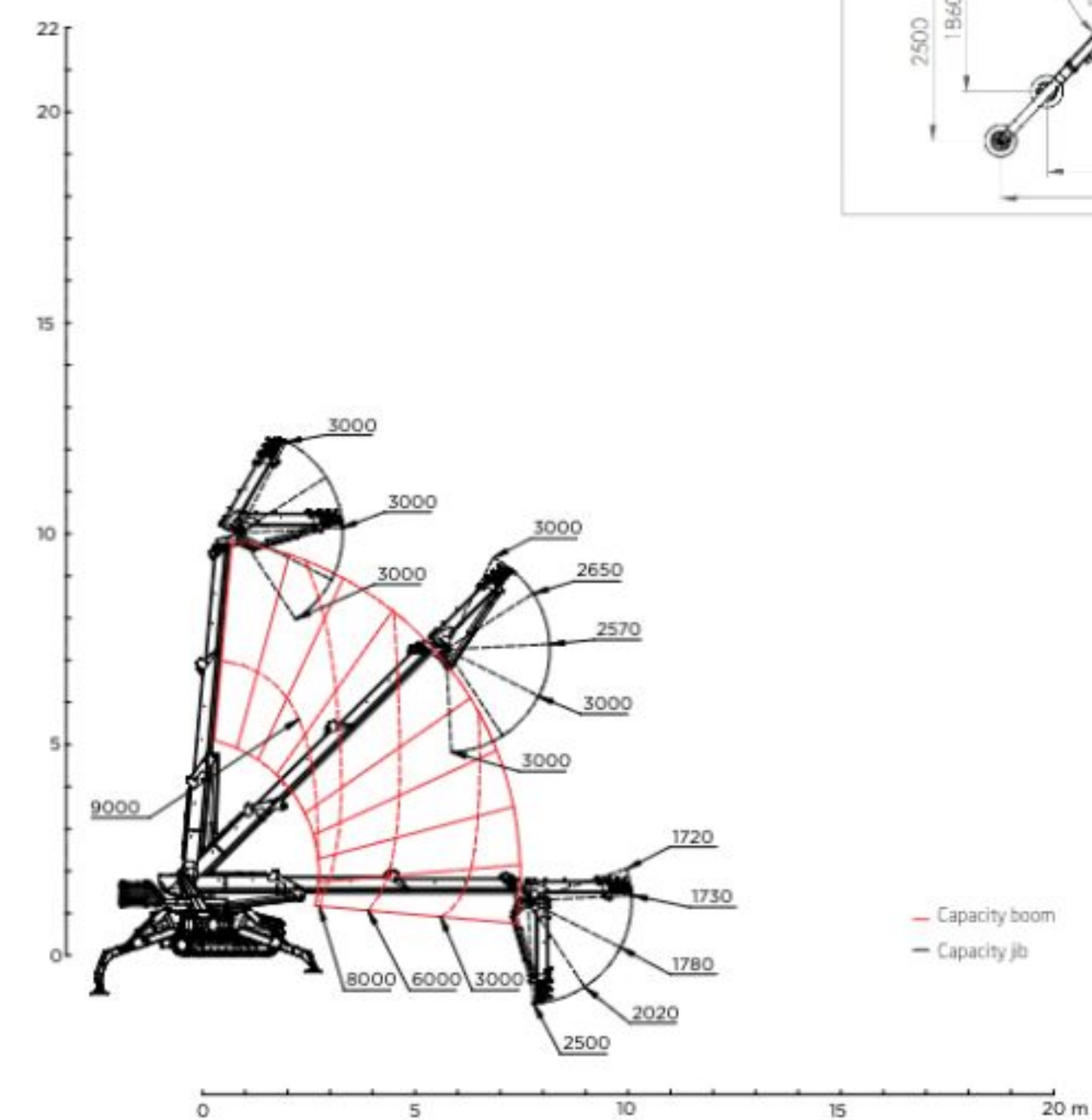
With chain locking system engaged
