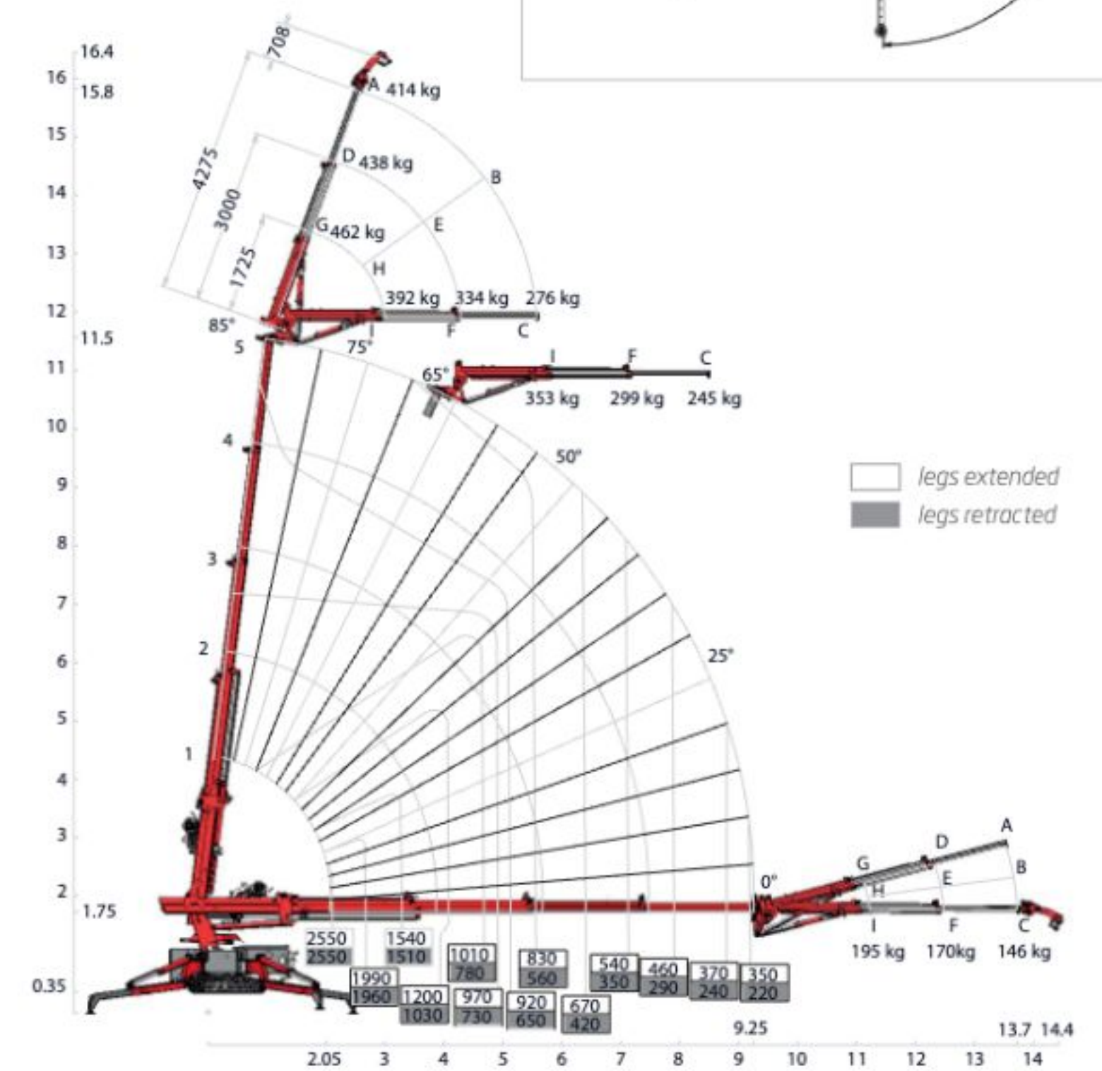
Without counterweight
