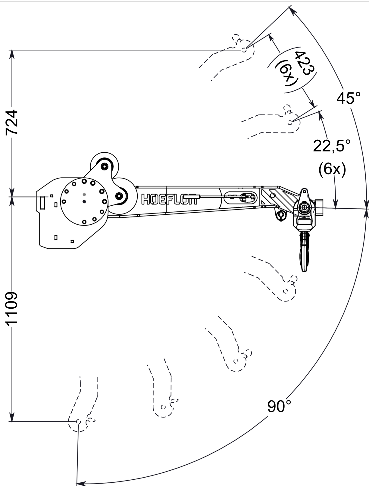
Tilt limits with lifting hook
