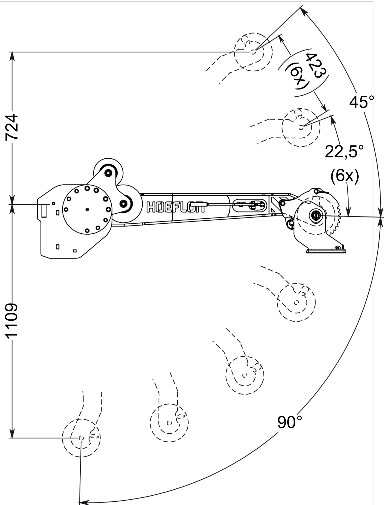
Tilt limits with winch head
